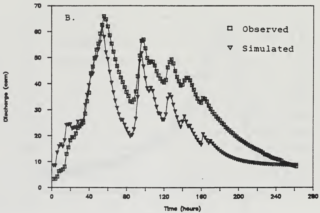
Figure 33. (A) Hyetograph, and (B) simulated and observed hydrographs for a "complex" rainfall event on the Nestucca River, Oregon Coast Range (February 14-28, 1968).
